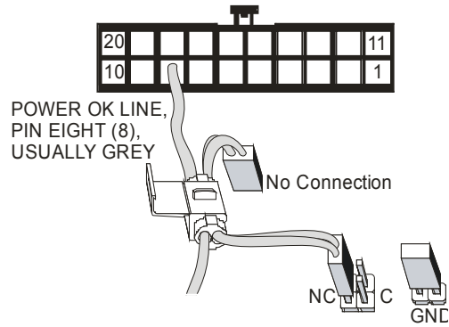
Figure 2-2: ATX Power Good Connection
