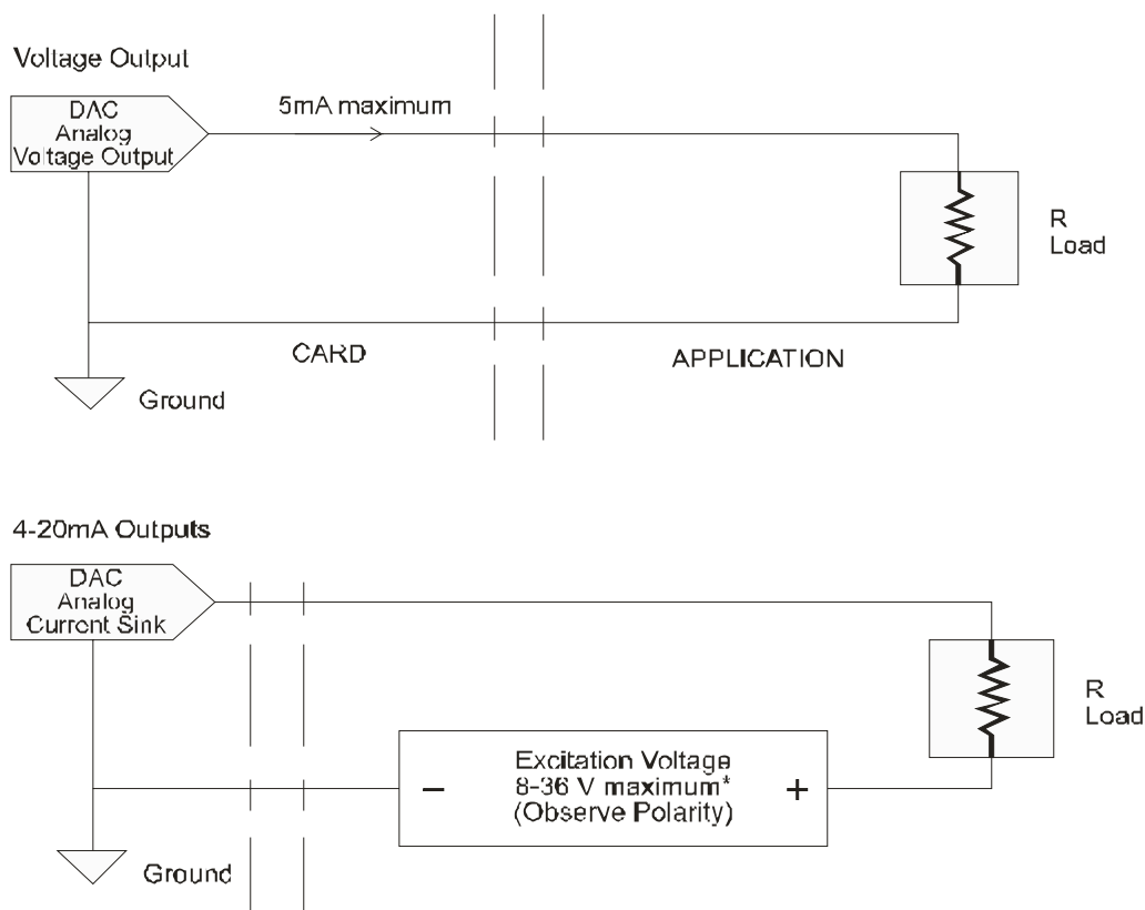
Figure 6-1: Signal Connection
